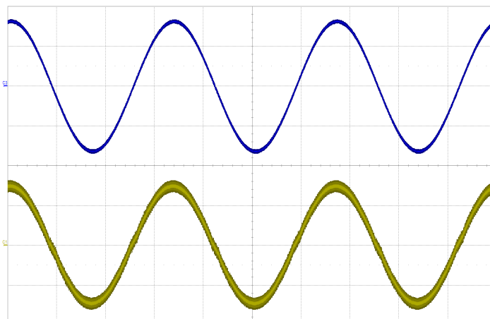
Figure 5: Typical Input Voltage and Current waveforms at full load current (115Vrms, 60Hz) Top: V_{in} (100V/div), Bottom: I_{in} (1A/div), Timebase: (5ms/div).
